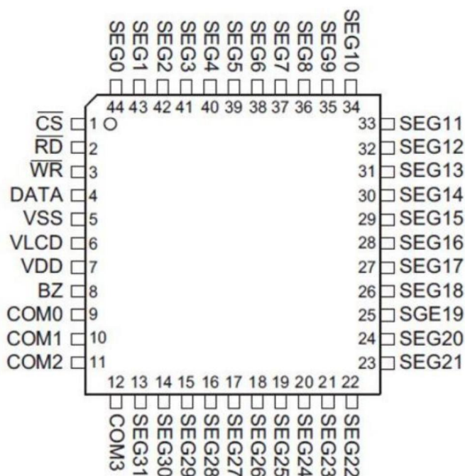
LQFP-44
