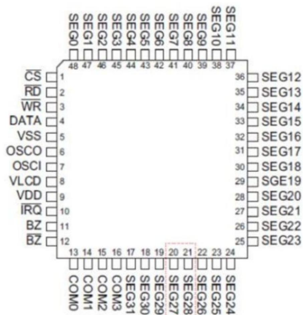
LQFP-48
