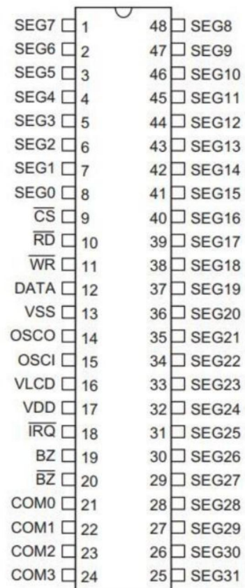
SSOP-48
